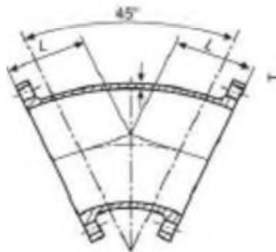
30 45° Double-flanged bends
