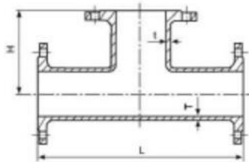
33 All-flanged tees
